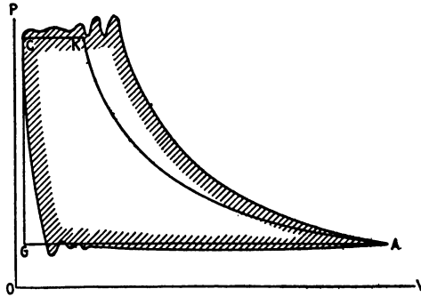
FIG. 46.—Cylinder efficiency.
